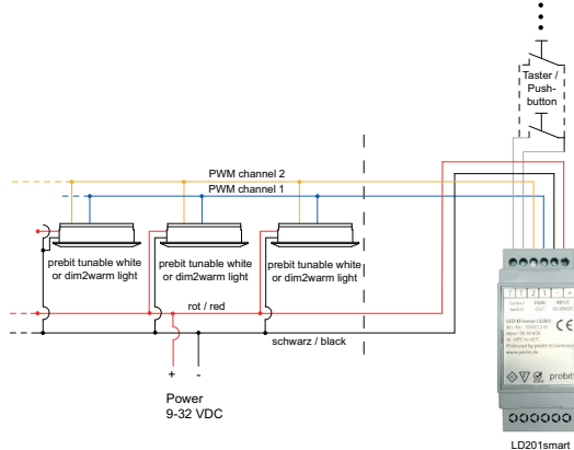
Profile tunable white or dim2warm (2-channel):
