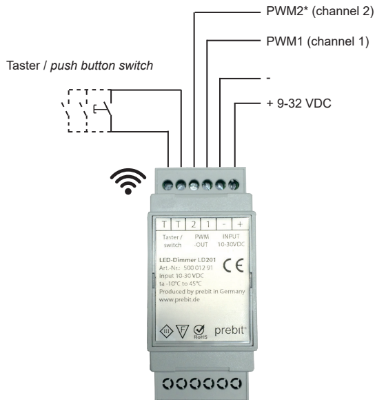
Profile tunable white or dim2warm (2-channel):
